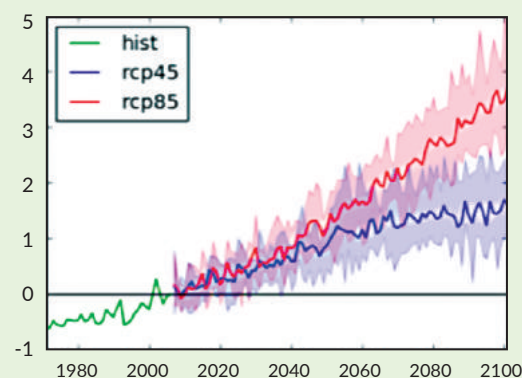
FIGURE 37: Projected Changes in Temperature for RCP 4.5 and RCP 8.5 relative to year 2000
