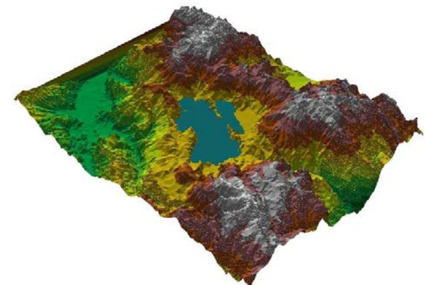
Digital elevation model of Tota Lake Watershed Source: Modified from the Plan of Organization and Management of Tota Lake. 2004
